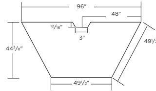
96"W TRAPEZOID COMPUTER TABLE
