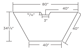
80"W TRAPEZOID COMPUTER TABLE
